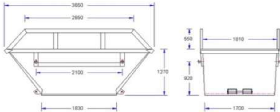
9m 3 Bin Dimensions
