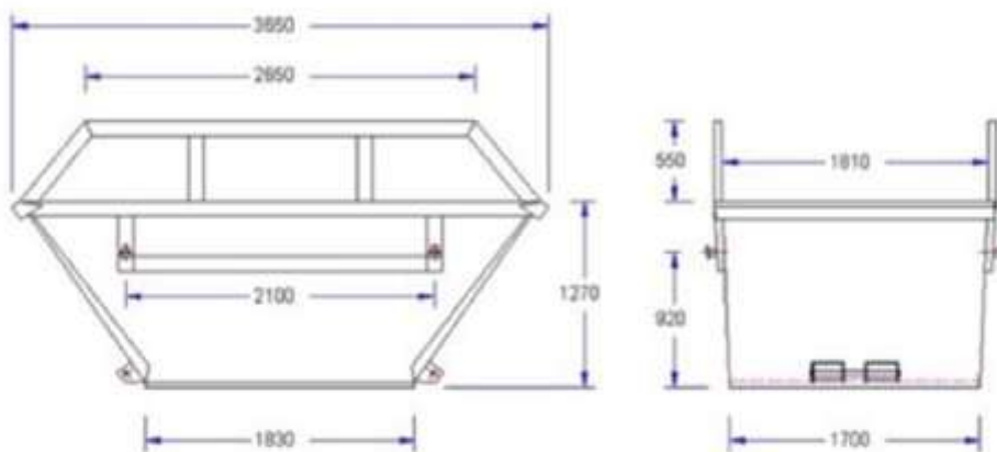
9m 3 Bin Dimensions
