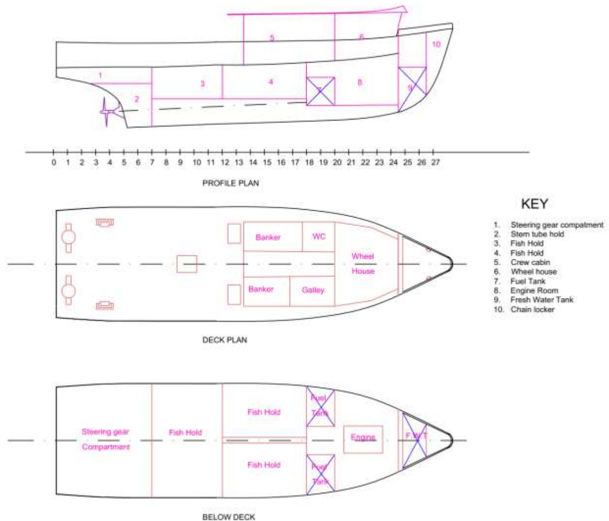
Typical Proposed Fishing Boat for KEMFSED Project
