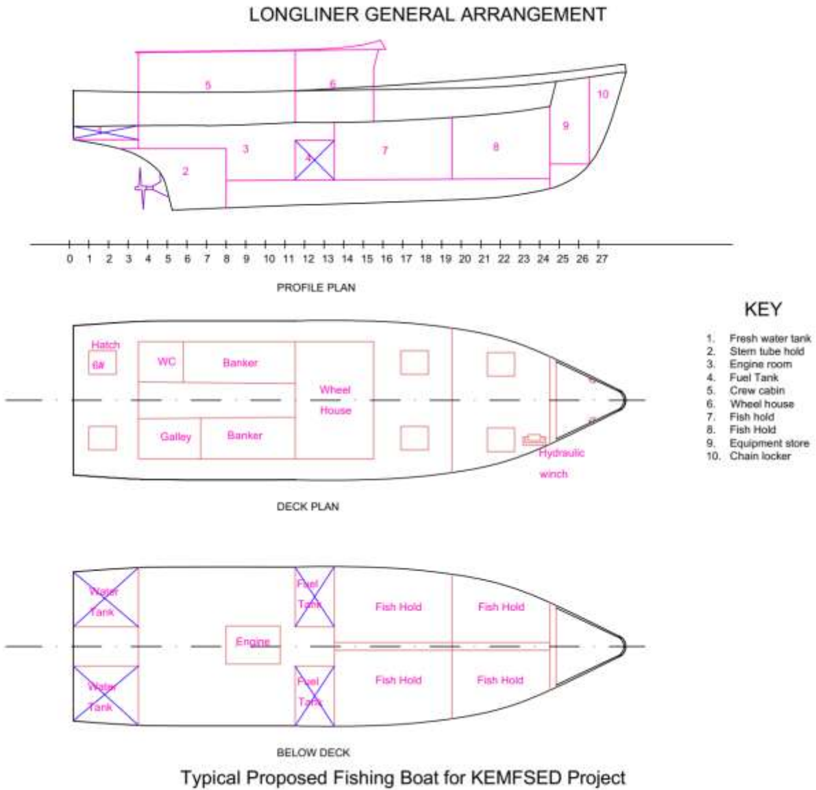
Figure 2: General arrangement for the recommended long line fishing boat
