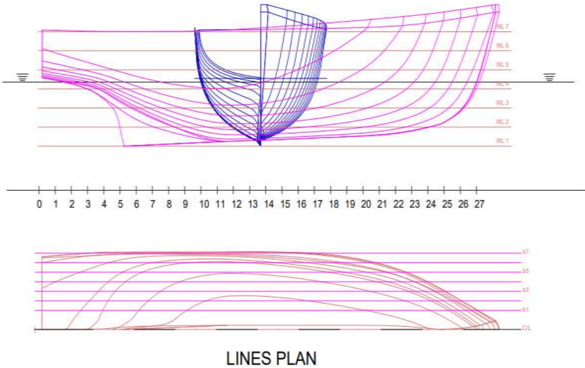
Typical Proposed Fishing Boat for KEMFSED Project
