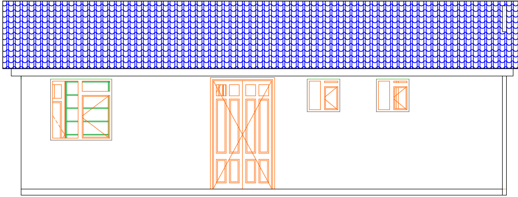
ELEVATION 01 SCALE 1: 50
