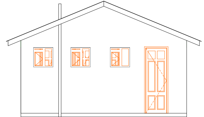
ELEVATION 04 SCALE 1: 50
