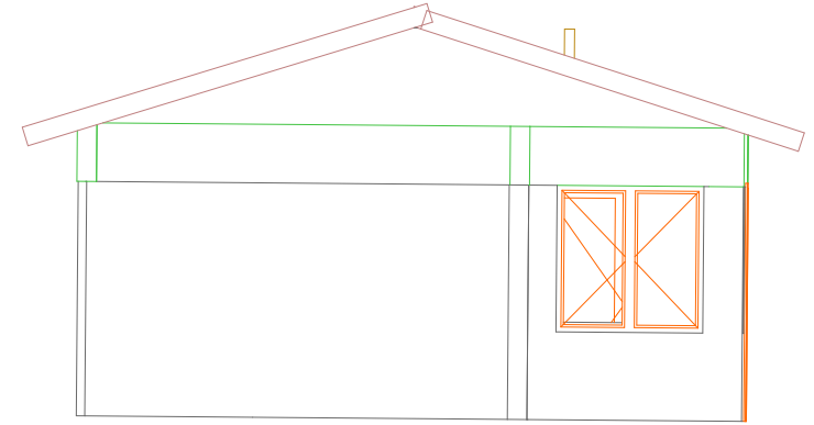
ELEVATION 02 SCALE 1: 50
