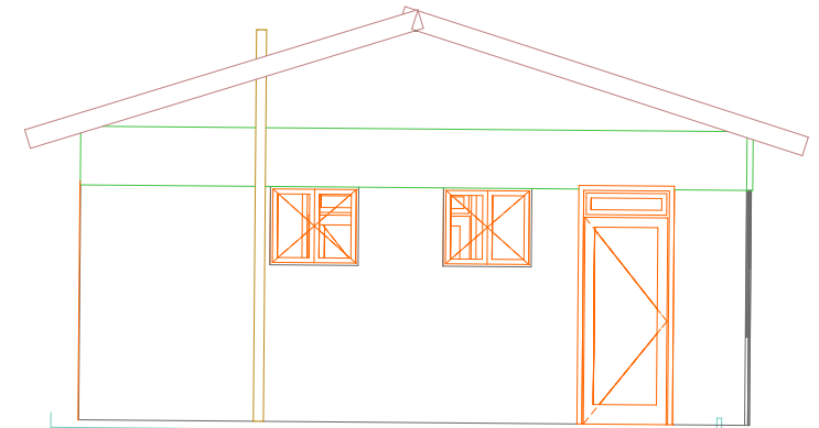
ELEVATION 04 SCALE 1: 50
